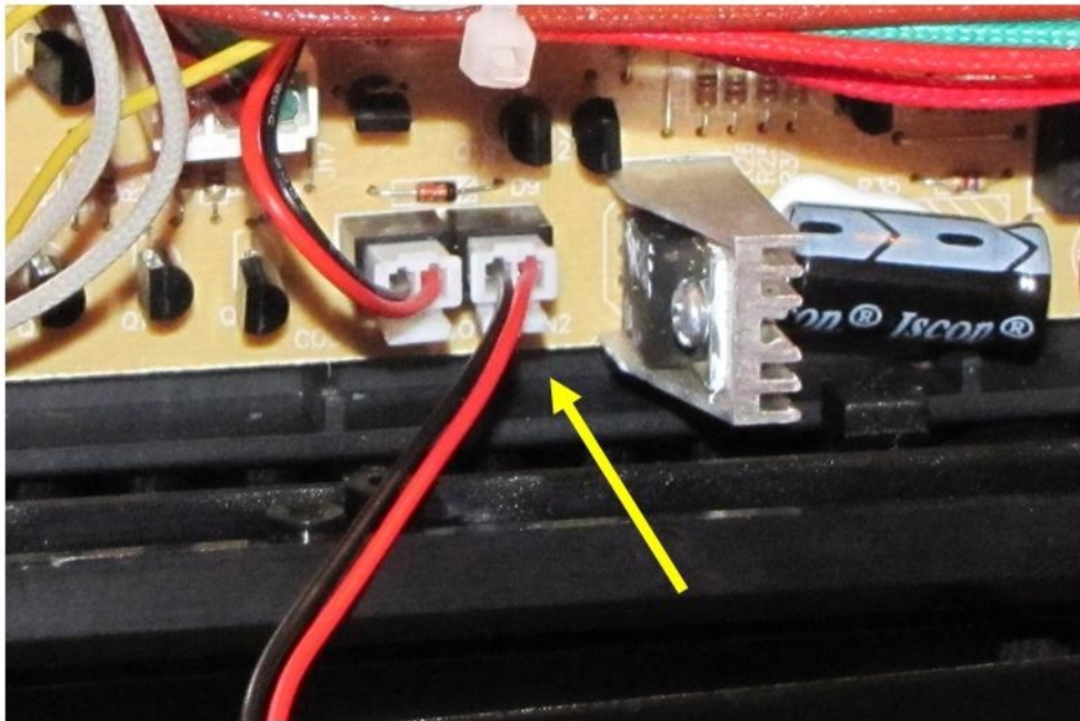
Lay panel flat beside the roaster. Insert male connector into the opening on the PCB (yellow arrow). Note the male connector has a tiny tab. That tab is to be downward as shown. Press Cool for a quick test, then re-assemble by gently lifting the panel and easing it back in place. Then replace the screws.
