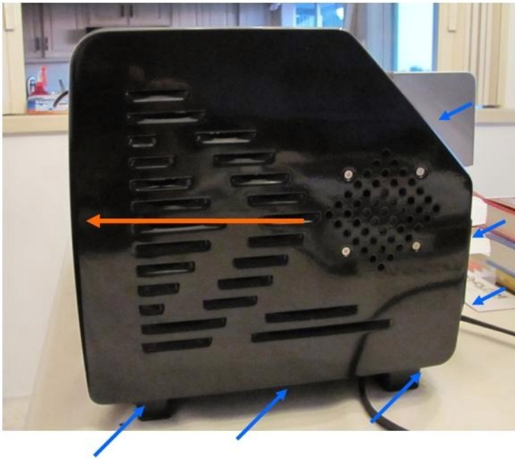
Remove 6 screws (blue arrows), slide panel forward (orange arrow) set panel aside
